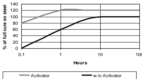
Cure Speed vs Activator
