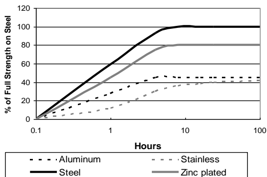
Cure Speed vs Substrate
