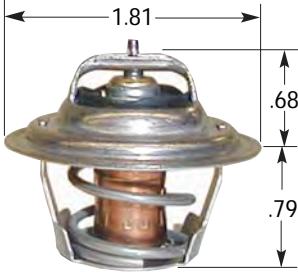
JIGGLE PIN IN VALVE
