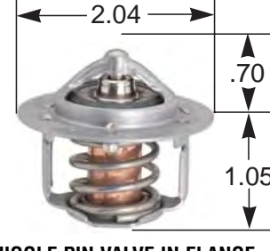
JIGGLE PIN VALVE IN FLANGE
