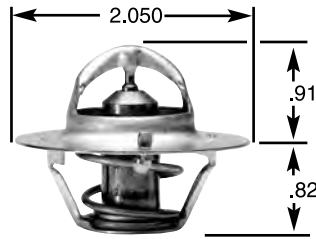
JIGGLE PIN VALVE IN FLANGE
