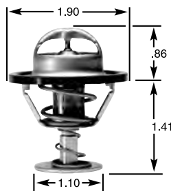
JIGGLE PIN VALVE IN FLANGE
