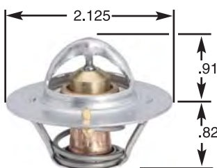
JIGGLE PIN VALVE IN FLANGE
