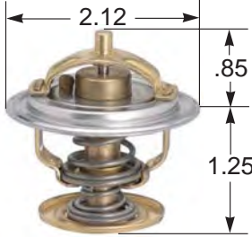
JIGGLE PIN VALVE IN FLANGE
