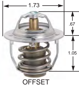
OFFSET JIGGLE PIN VALVE IN FLANGE
