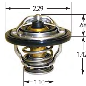
JIGGLE PIN VALVE IN FLANGE
