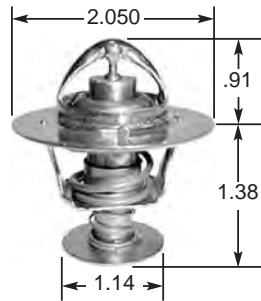
JIGGLE PIN VALVE IN FLANGE
