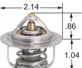
JIGGLE PIN VALVE IN FLANGE
