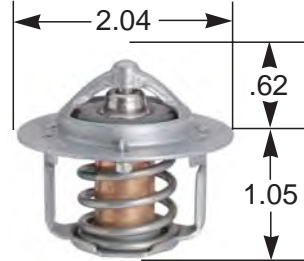
JIGGLE PIN VALVE IN FLANGE
