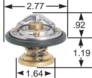
JIGGLE PIN VALVE IN FLANGE
